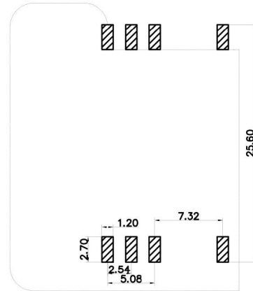
RECOMMEND P. C. BOARD LAYOUT
